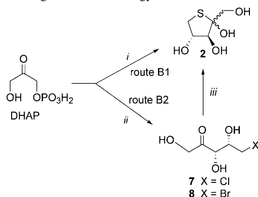
Scheme 5. FruA-catalysed aldolisation reaction from DHAP; i: a: (C 2 H 4 SO) 2 , FruA, pH 7.5, b: acid phosphatase (Pase), pH 4.7, 60%; [18] ii: a: XCH 2 CHO, FruA, pH 7.5, b: Pase, pH 4.7, 71% ( 7 ) or 55% ( 8 ); iii: Na 3 SPO 3 , 55% (from 7 or 8 ); or NaSH, 57% (from 7 ) or 61% (from 8 ).
