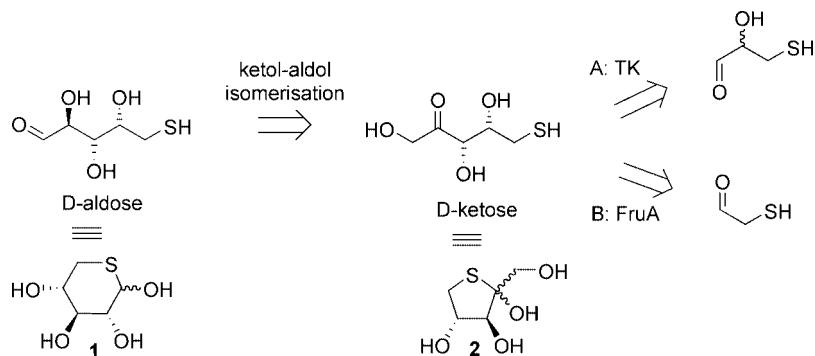
Scheme 3. The 5-thio-D-xylopyranose retrosynthetic pathway; Route A: catalysed by transketolase (TK), Route B: catalysed by fructose-1,6-bisphosphate aldolase (FruA).
