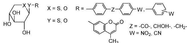
Scheme 1. 5-Thio-D-xylopyranosides derivatives tested as oral venous antithrombotics.
